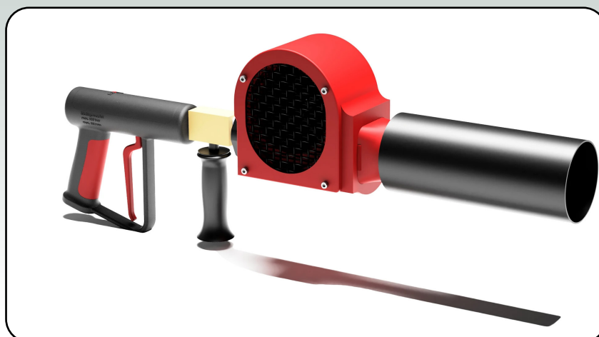
FoamGiant standard version for firefighting systems with integrated foam agent injector
